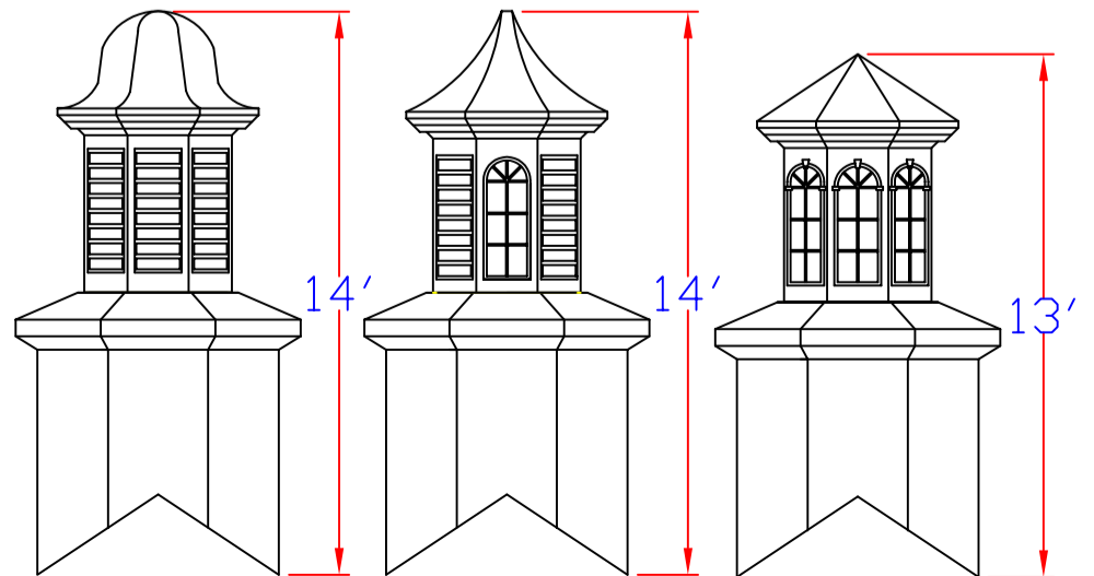
870-LR 870-LWP 870-WPK 800 Series 6' Octagon Base Models
