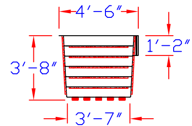
End View
