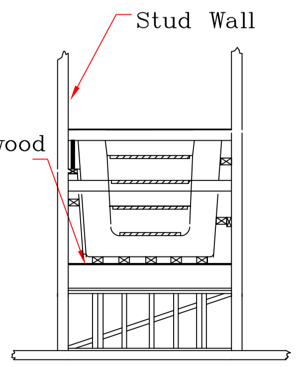
End View Showing Step Bracing
