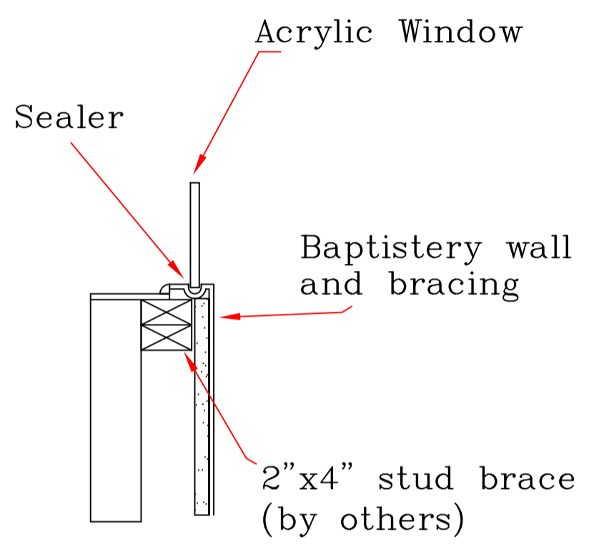
Window Detail
