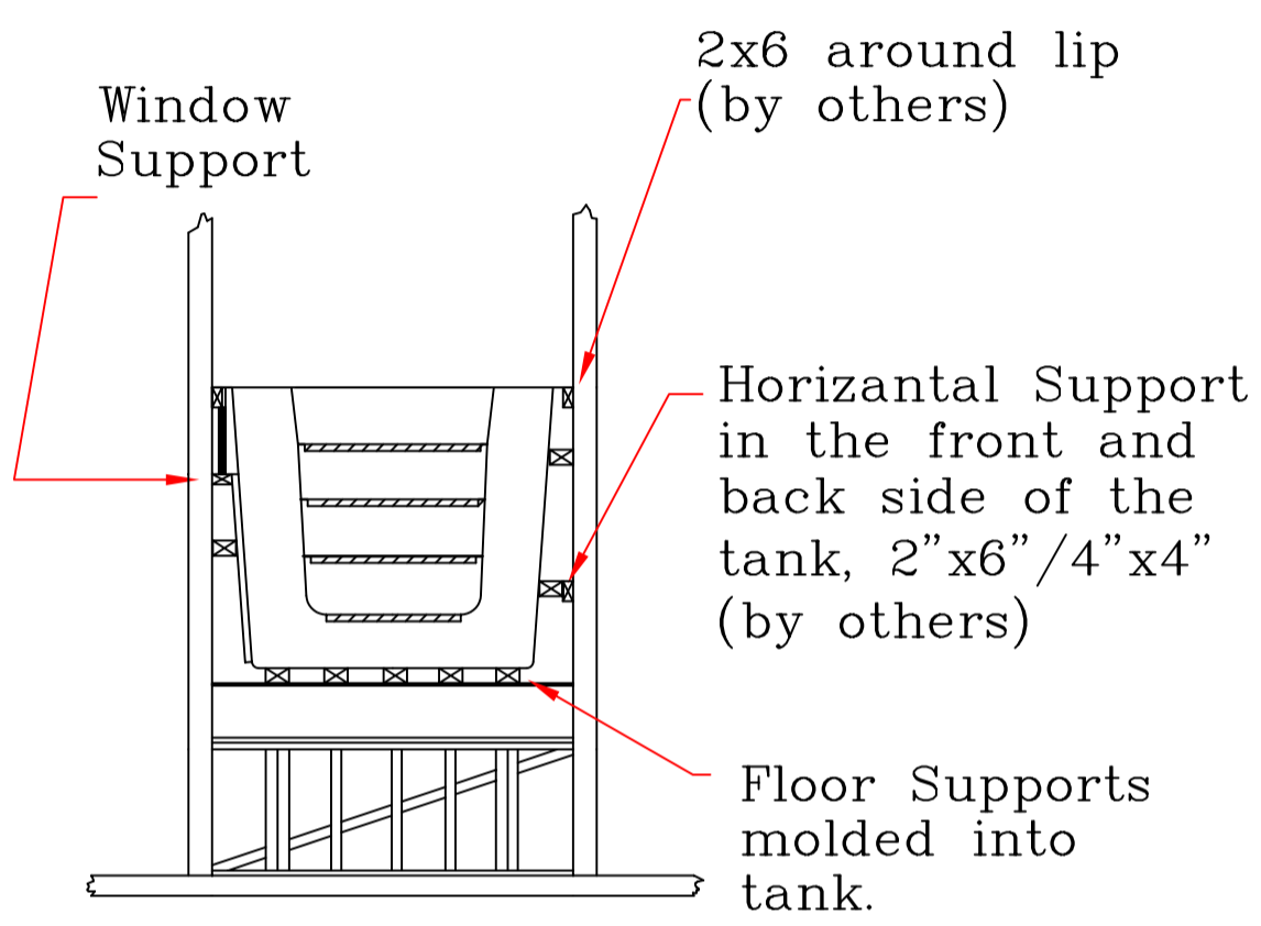
End View
